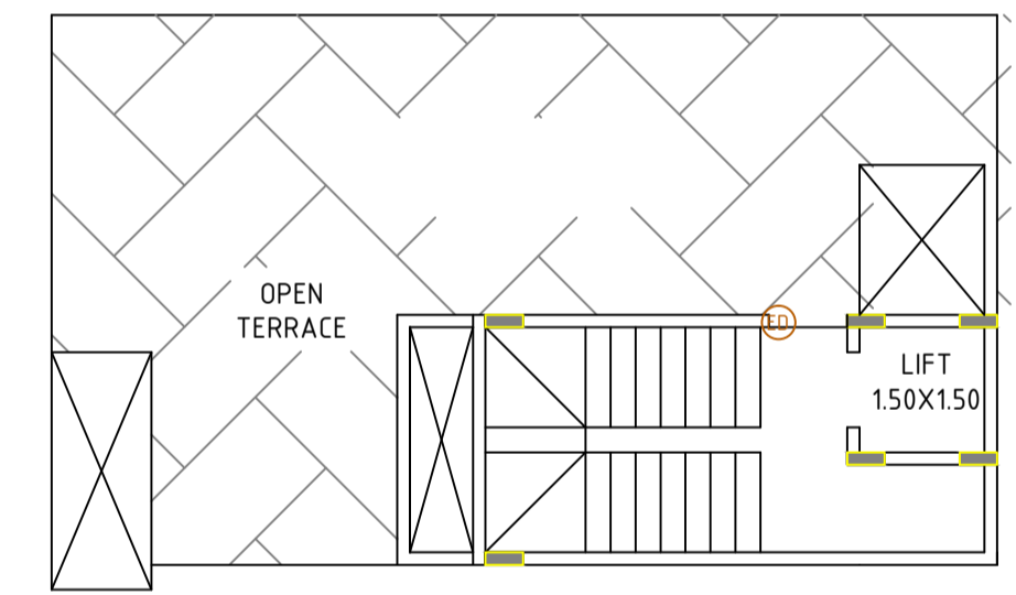
TERRACE FLOOR PLAN (1:100)
