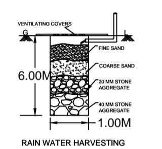
RAIN WATER HARVESTING STRUCTURE DETAILS
